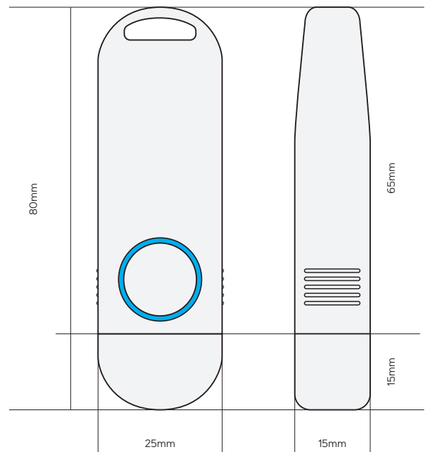
Example: Custom ONEKEY with one button interface
